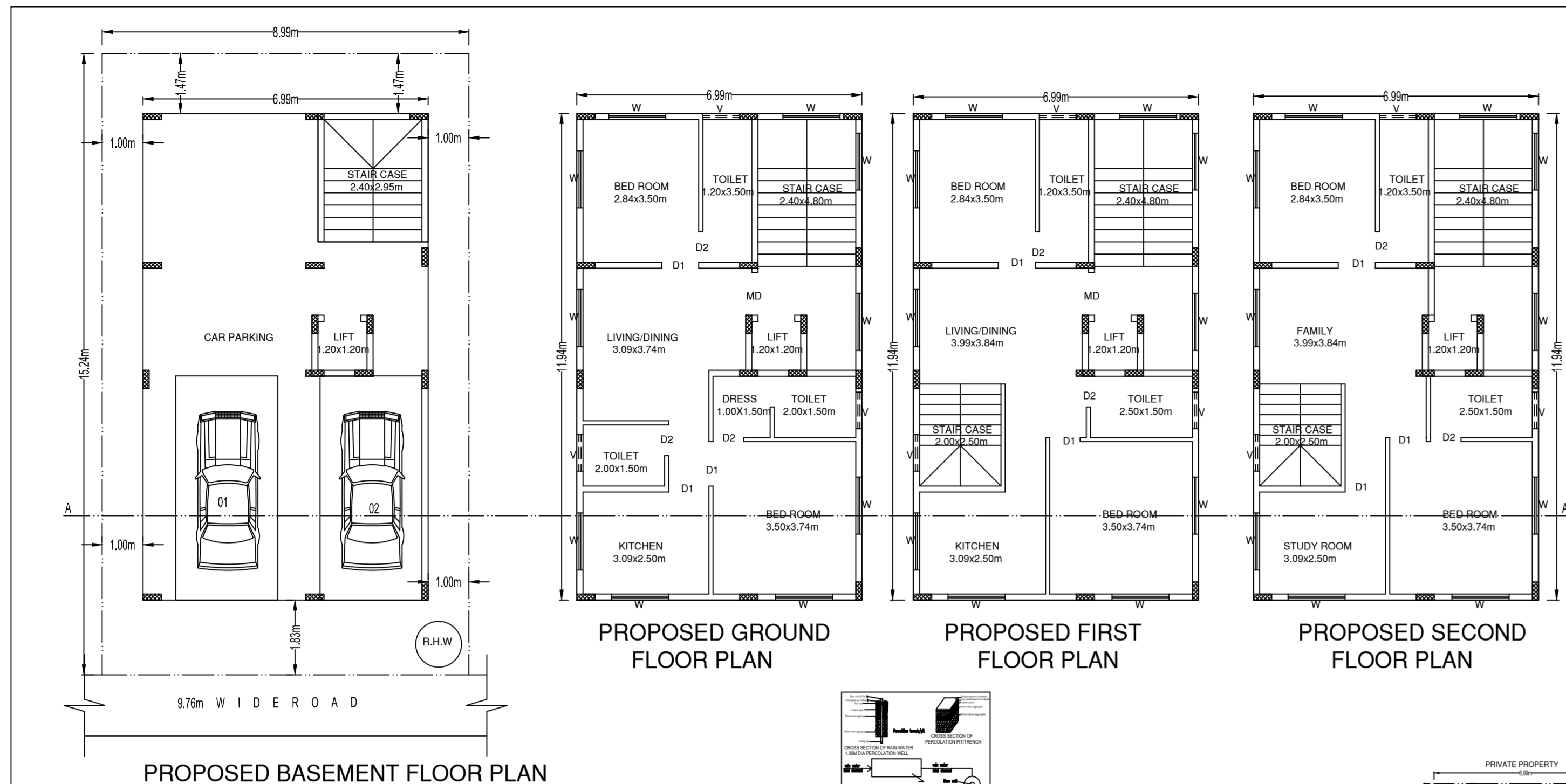
PROPOSED BASEMENT FLOOR PLAN
